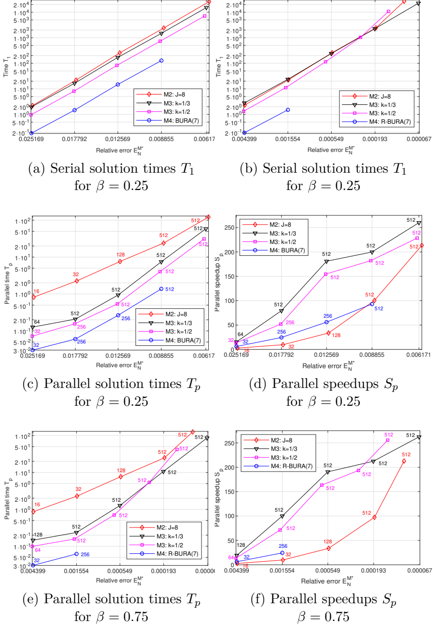
Figure 2.6: Comparison of parallel numerical algorithms for selected methods (M2)–(M4) solving the 3D test problem (2.16)–(2.17)
